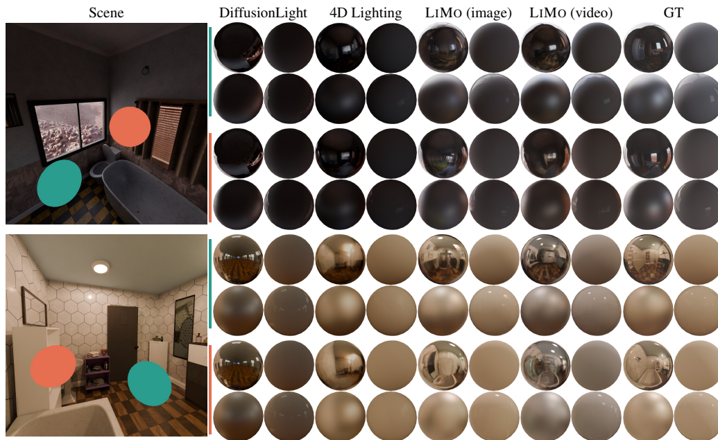
Figure 4. Sample predictions from the Infinigen test set [32] for, from left to right: DiffusionLight [31], 4D Lighting [42], and the image and video versions of the proposed LiMO. We visualize predictions by rendering the same four test spheres used for the quantitative metrics (see Tab. 2): mirror (top left), diffuse (top right), matte (bottom left) and glossy (bottom right).
