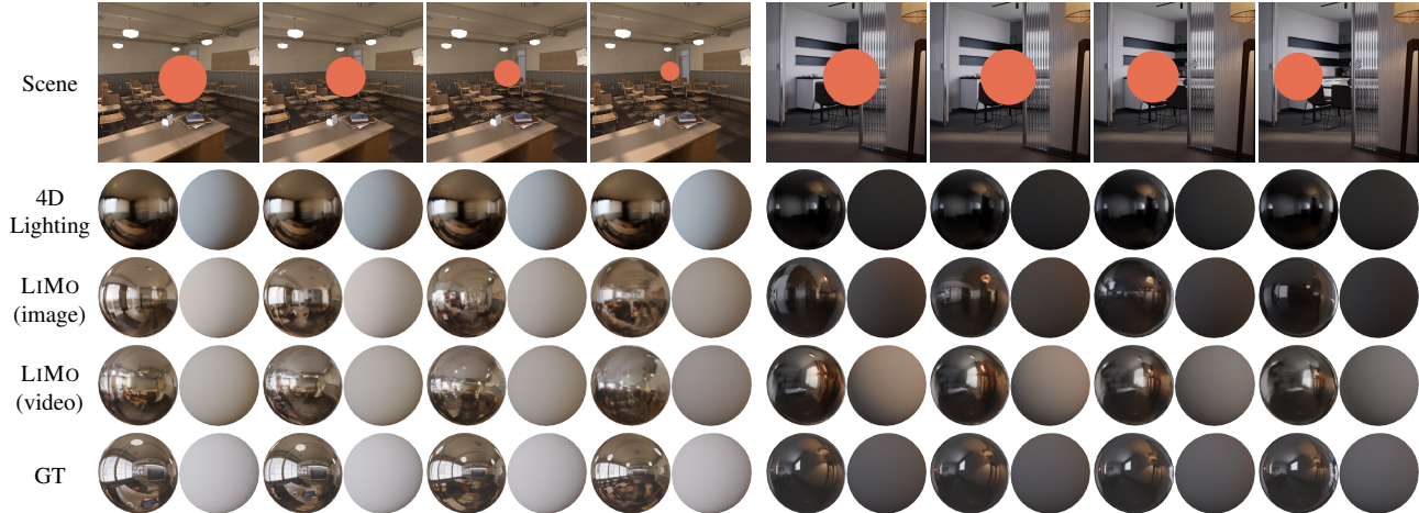
Figure 5. Example qualitative prediction results on our proposed video test set. Observe how our predictions are more detailed and more closely match the ground truth than the previous work 4D Lighting [42] as the sphere moves around the scene.
