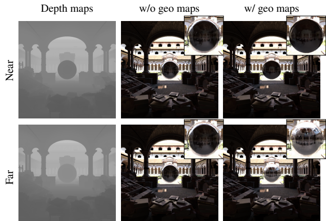
Figure 6. The effect of our proposed geometric maps \{I_{dir}, I_{dist}\} . We insert a sphere near (top) and far (bottom). Observe how the addition of geometric maps (right) helps the network in reasoning about light occlusions, which are not captured otherwise (middle).
