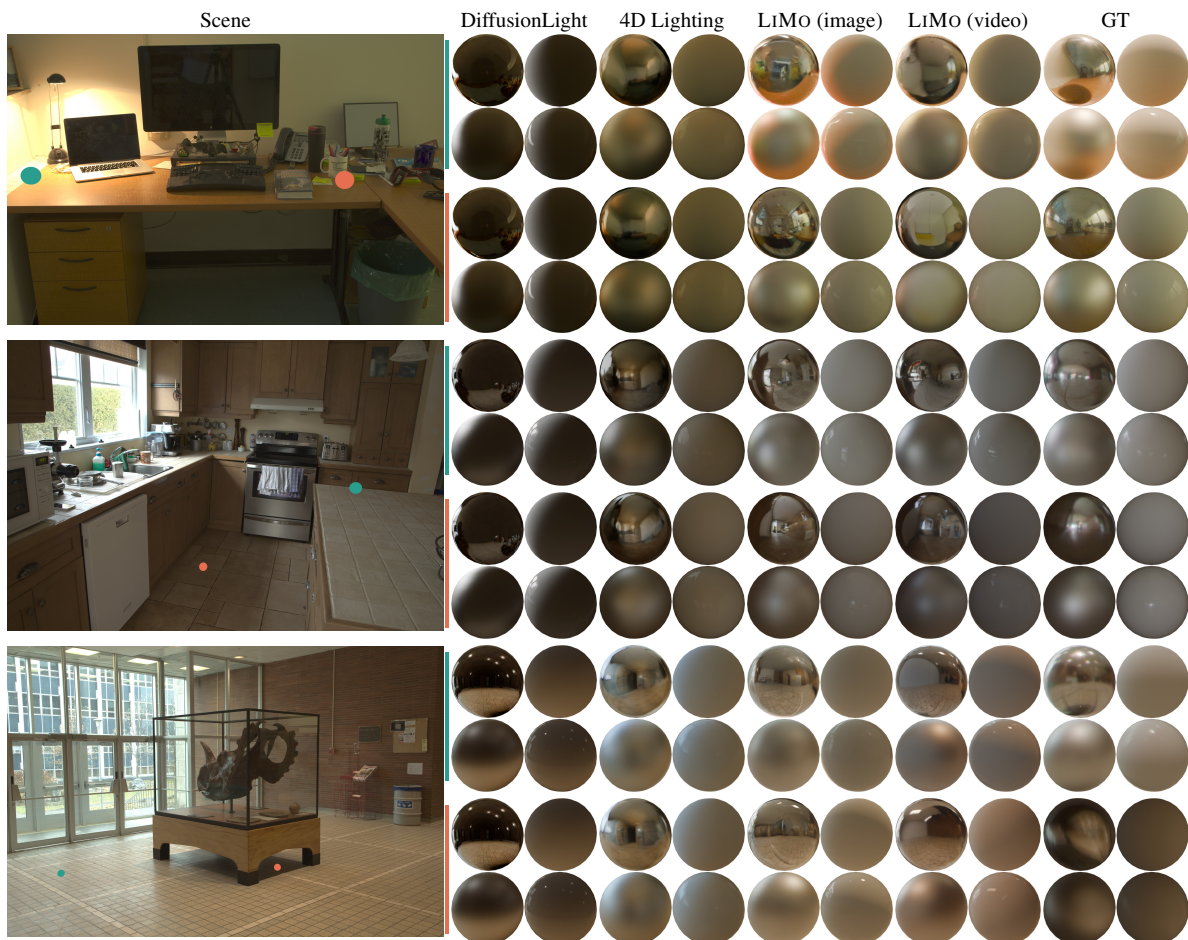
Figure 8. Additional sample predictions from the Laval Indoor Spatially Varying test set [17] for, from left to right: DiffusionLight [31], 4D Lighting [42], and the image and video versions of the proposed LiMO. We visualize predictions by rendering the same four test spheres used for the quantitative metrics (see Tab. 2): mirror (top left), diffuse (top right), matte (bottom left) and glossy (bottom right).
